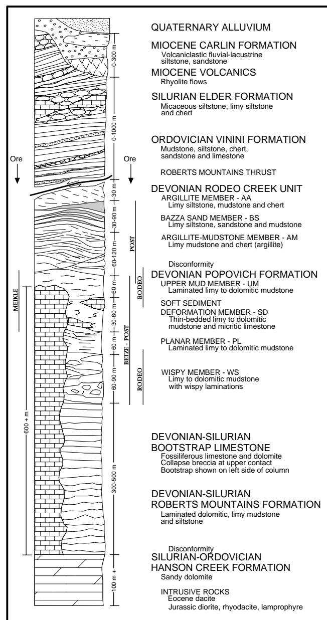
Figure E-4. Stratigraphic column of the Goldstrike property, showing relationship of major orebodies and stratigraphic units. Modified from Bettles and Lauha (1991) and Volk and others (2001).
