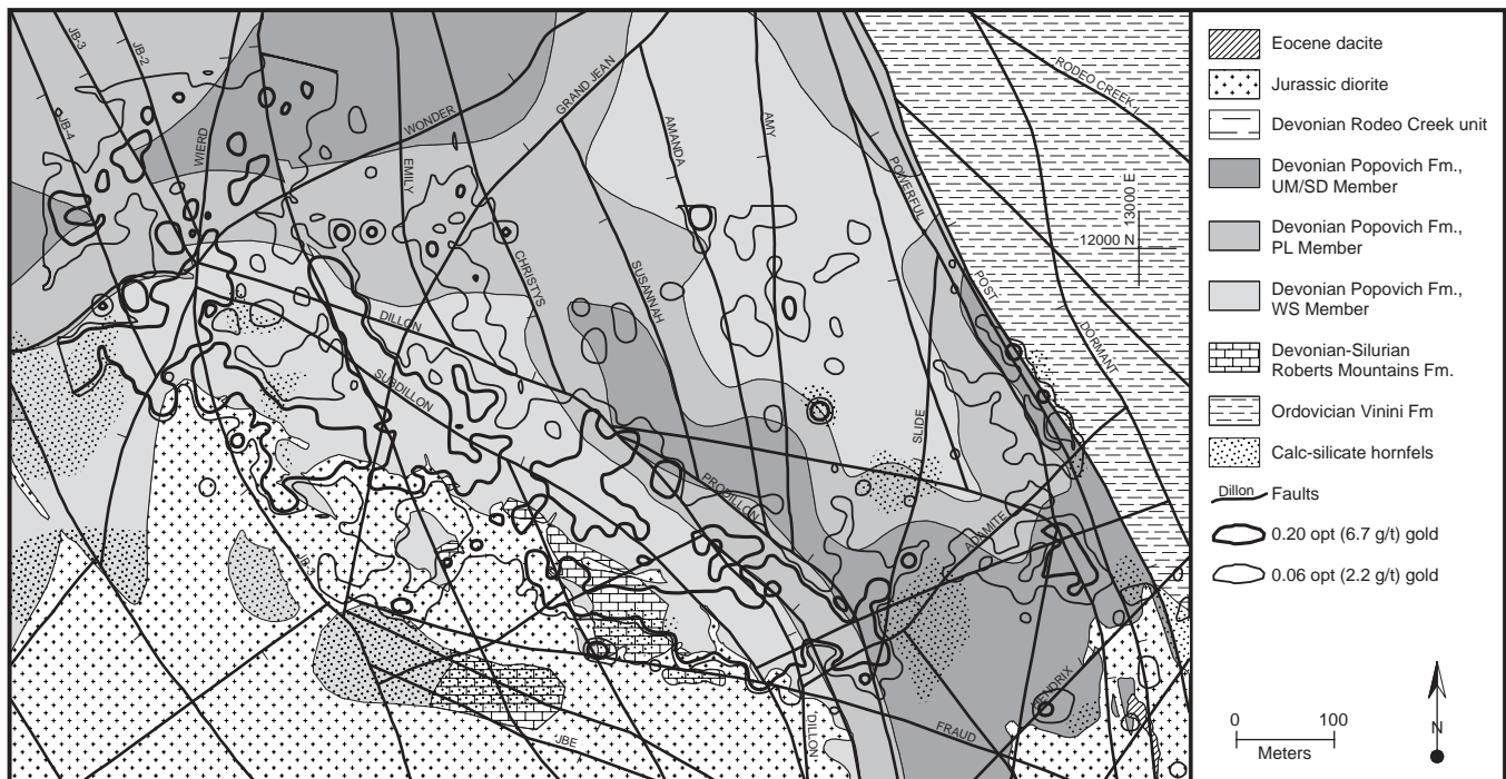
Figure E-9. Level plan at the 4700 level (1,433 m) of the Betze and Deep Post subdeposits of the Betze-Post deposit. Important ore controls shown at this level are the Wispy Member of the Popovich Formation, the Dillon fault zone, and the contact of the Jurassic diorite. Small displacements on faults are not shown. The location of the level plan is shown in figure E-5.
