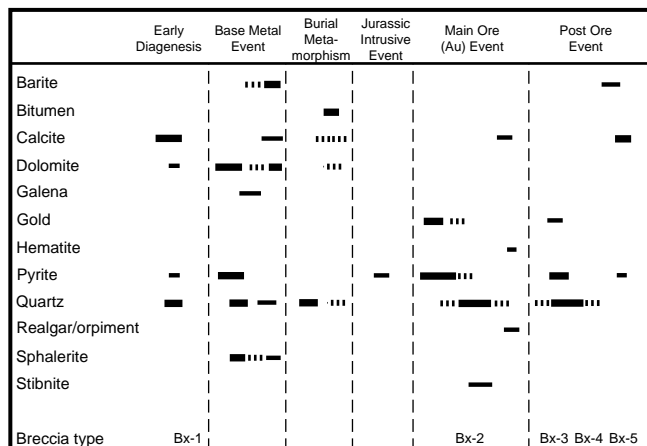
Figure E-7. Mineral paragenesis at the Meikle deposit. From Evans (2000).
